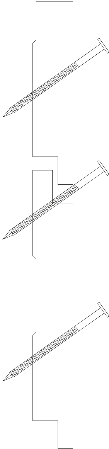
SHIPLAP NAIL (FACE NAIL)
